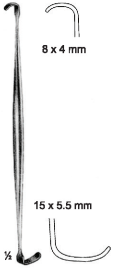
RAGNELL-DAVIS OI 16-4201-14 14 cm/5 1/2"
